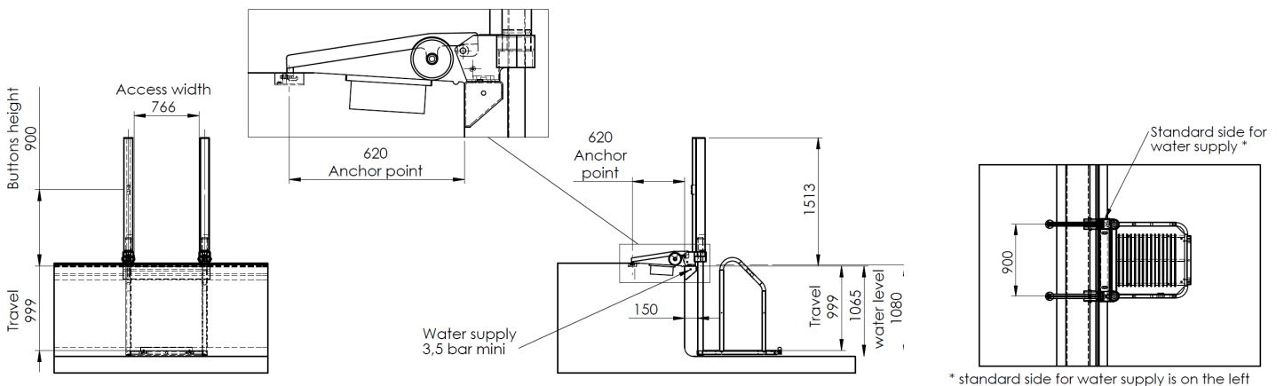
DETAIL A
