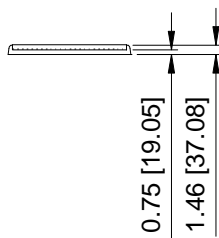
TOE END VIEW
